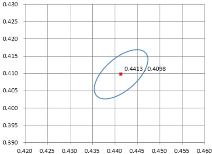
Chromaticity Bins: 1931 CIE Curve
